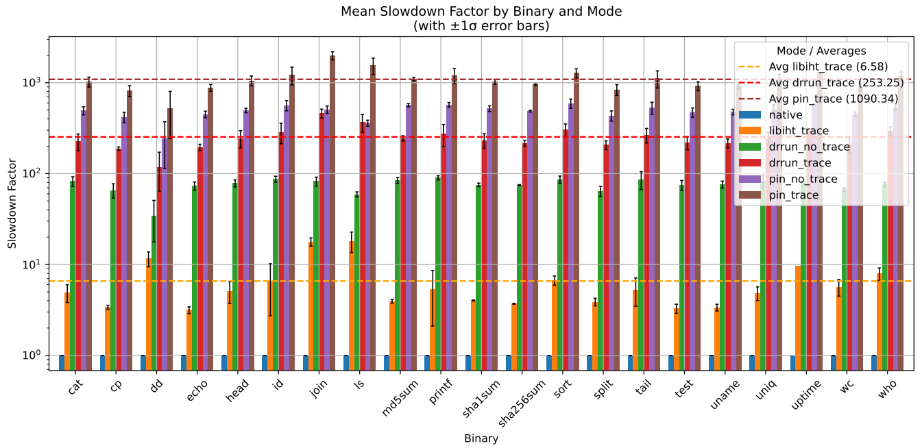
Figure 6: Average slowdown factors for standard Unix command-line utilities relative to native execution across six modes. Dashed horizontal lines denote the overall mean slowdown across the benign benchmark
