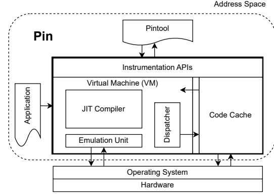
Figure 1: High-level architecture of the Intel Pin (adapted from [18]). The tool inserts a virtual machine, JIT compiler, and dispatcher to dynamically transform the target program, storing instrumented code in a dedicated code cache.
