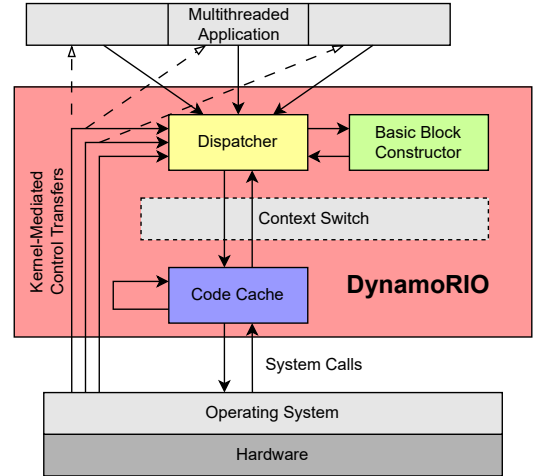
Figure 2: Overview of DynamoRIO’s architecture (adapted from [5]). Similar to Intel Pin, it uses a code cache for instrumented basic blocks, with a dispatcher managing control transfers to and from the running application.
